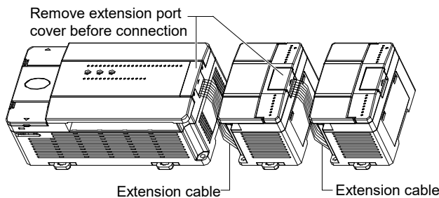
Figure 5-1 Cascade connection of extension module
