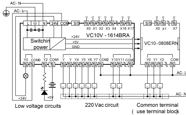
Figure 4-1 Connecting VC10V-1614BRA & VC10-0808ERN
